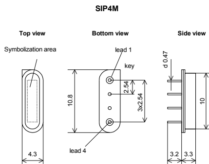
Dimensions in mm Mass 0.8 g
